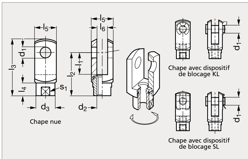
Chape de tringlerie acier 31-26 Page 1534
